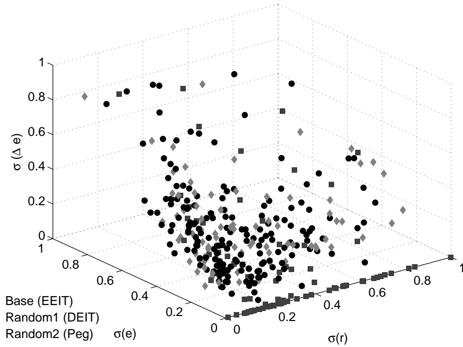
Figure 1: Random composition of the data sample (Step 1).
