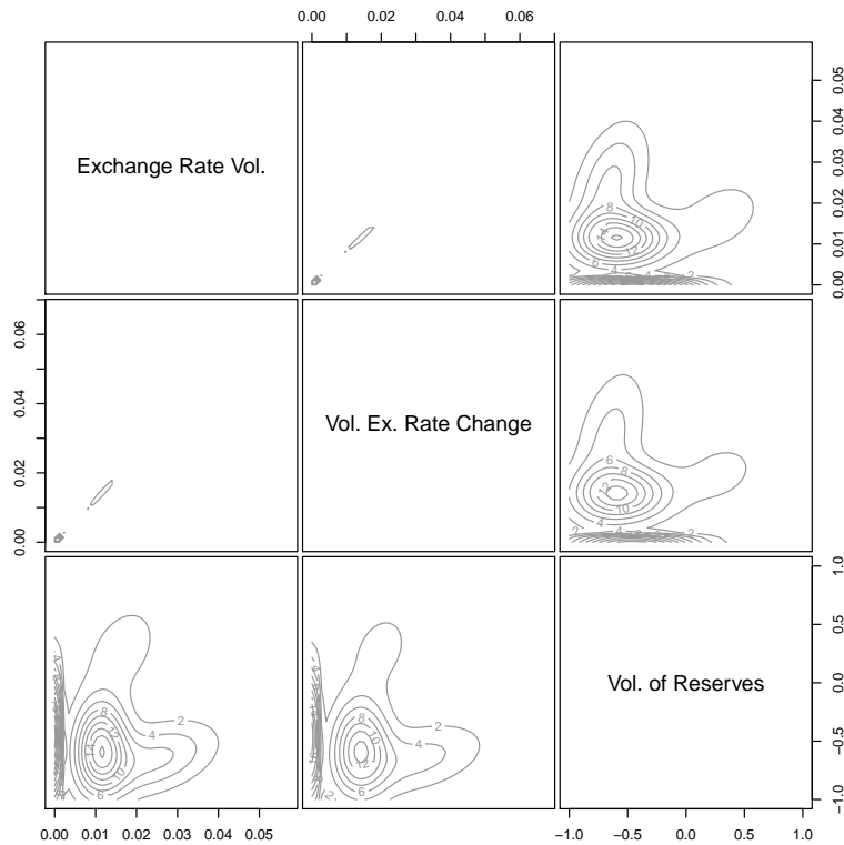
Figure 3: Correspondance between the optimal number of Gaussians and the number of modes appearing on the join density.
