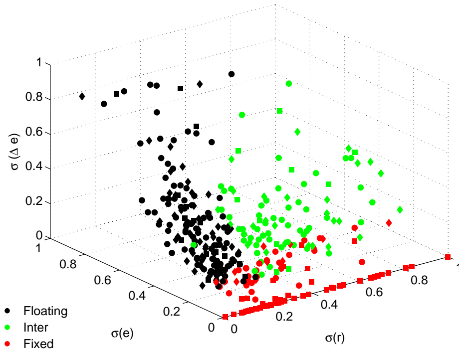
Figure 4: Labelling clusters as de facto regimes (Step 3).
